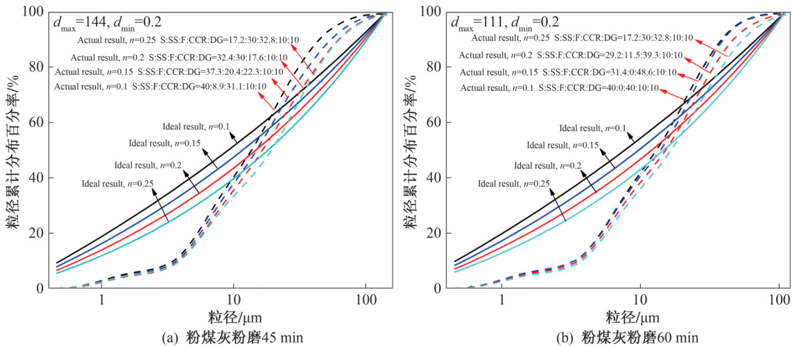
图 4 理想级配与真实级配对比结果 Fig. 4 Comparison results of ideal gradation and actual gradation
